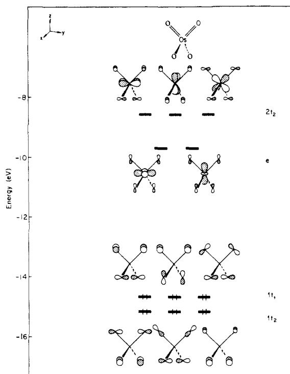
Figure 1. Valence orbitals of OsO 4 .
