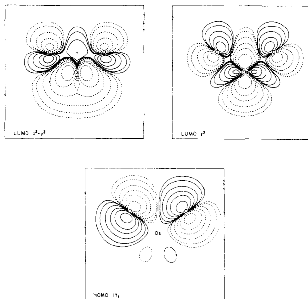
Figure 2. Plot of three of the valence orbitals of OsO 4 . The contour levels of \Psi are 0.2, 0.1, 0.055, 0.025, 0.01, and 0.005. The orbitals are plotted in the yz plane. The two upper plots are the LUMO's and the lower the HOMO.
